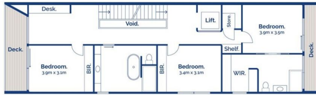
First Floor.
