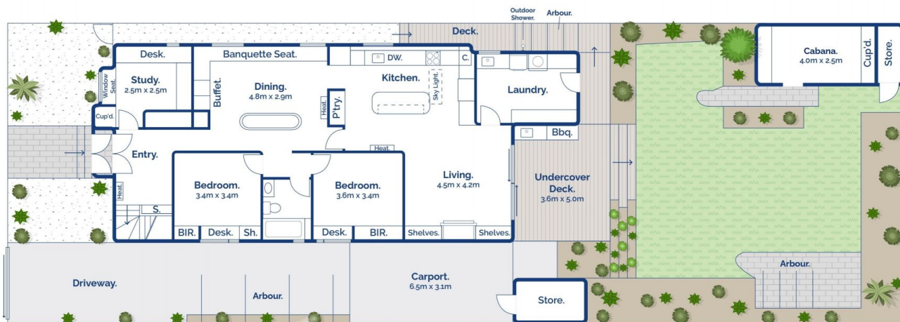
Ground Floor.
