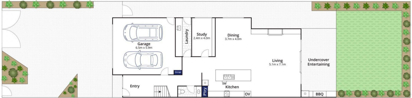
Ground Floor
