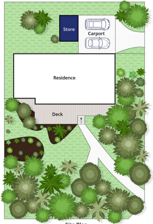
Site Plan
