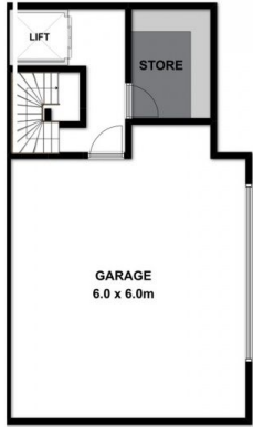
Ground Level
